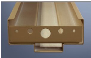
5 3/4" Frame (with returns)
